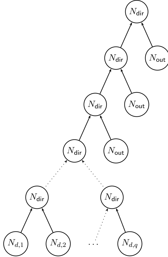
Figure 2: Illustration of the Definition of Sets \mathcal{N}_{\text{leaves}} , \mathcal{N}_{\text{dir}} , \mathcal{N}_{\text{out}} .
