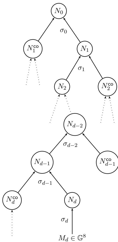
Figure 1: Illustration of the tree-based signature scheme. In this example we have M_0 = (N_1^{co}, N_1) , M_1 = (N_2, N_2^{co}) , \dots , M_{d-1} = (N_d^{co}, N_d) and M_d = M .
